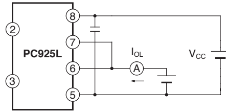
Fig.2 Test Circuit for Low Level Output Current
