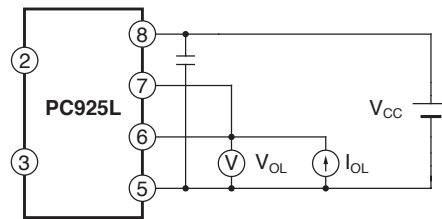
Fig.4 Test Circuit for Low Level Output Voltage
