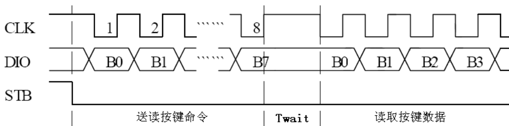
图7、数据读取
