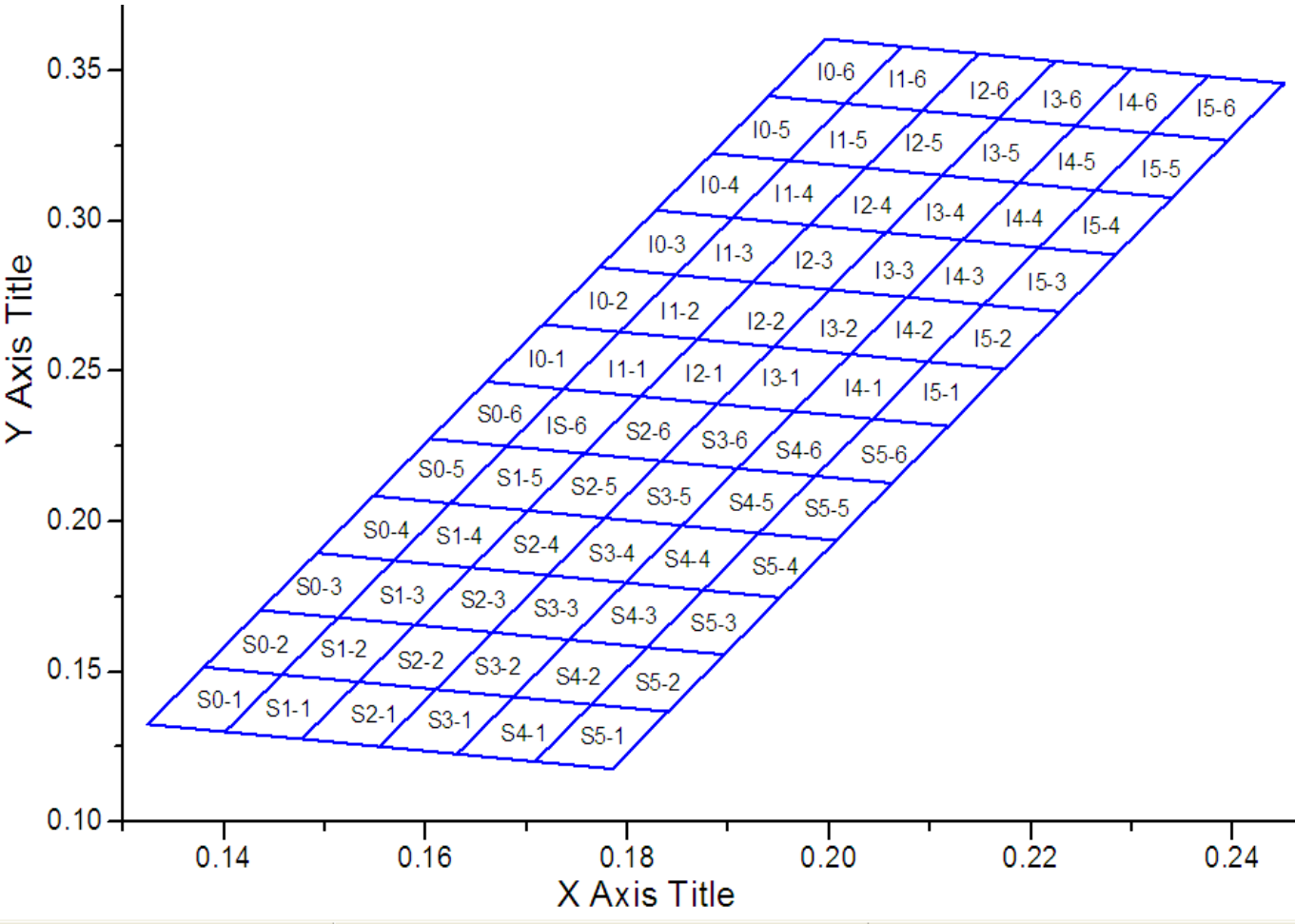
Chromaticity Diagram 2
