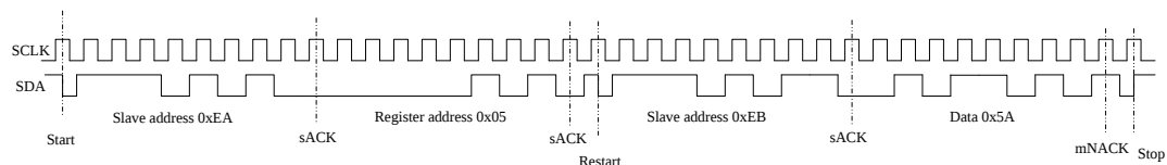
I2C Read
