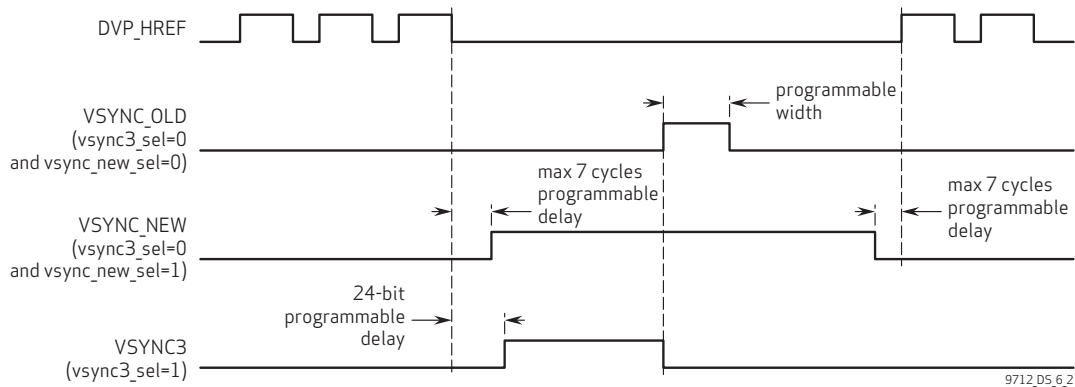
figure 6-2 VSYNC timing
