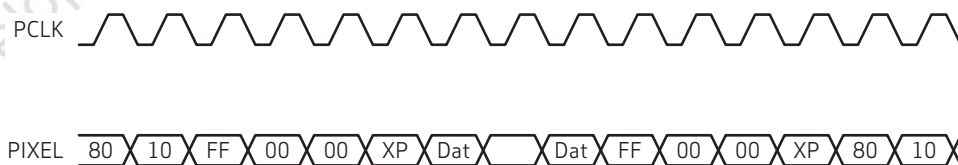
figure 6-3 CCIR656 timing
