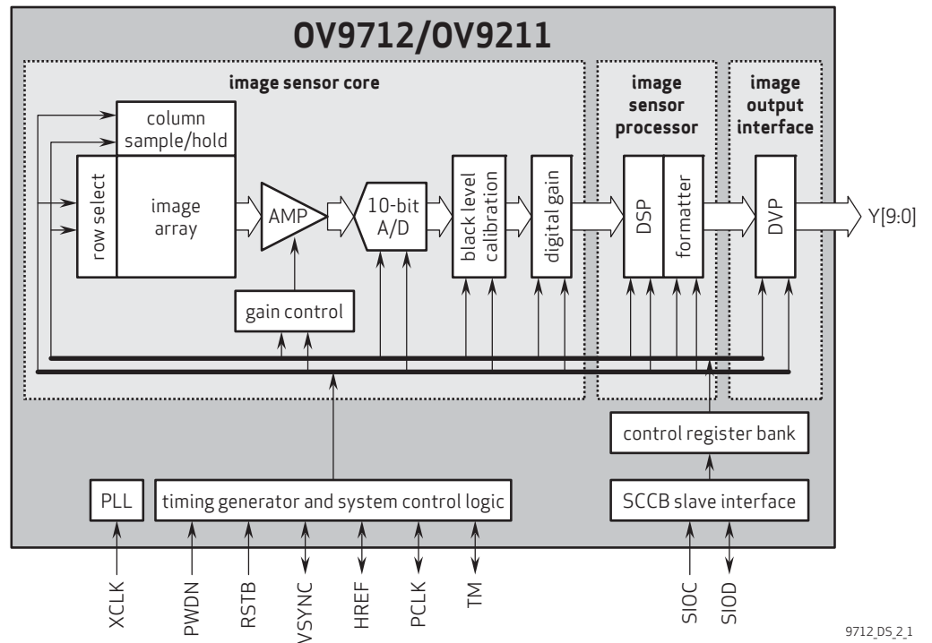
figure 2-1 OV9712/OV9211 block diagram
