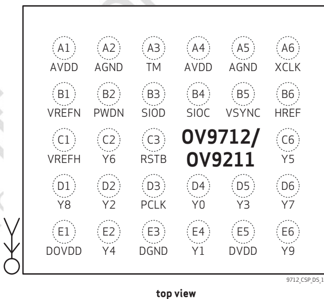
figure 1-1 pin diagram
