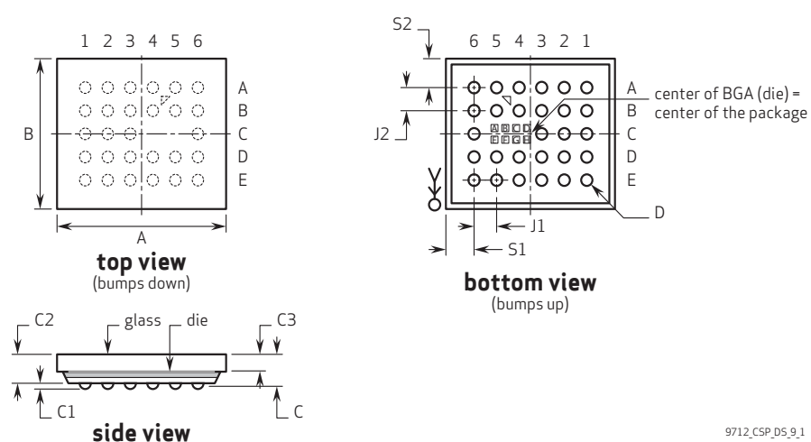
figure 9-1 package specifications
