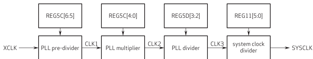
figure 2-3 system control block diagram
