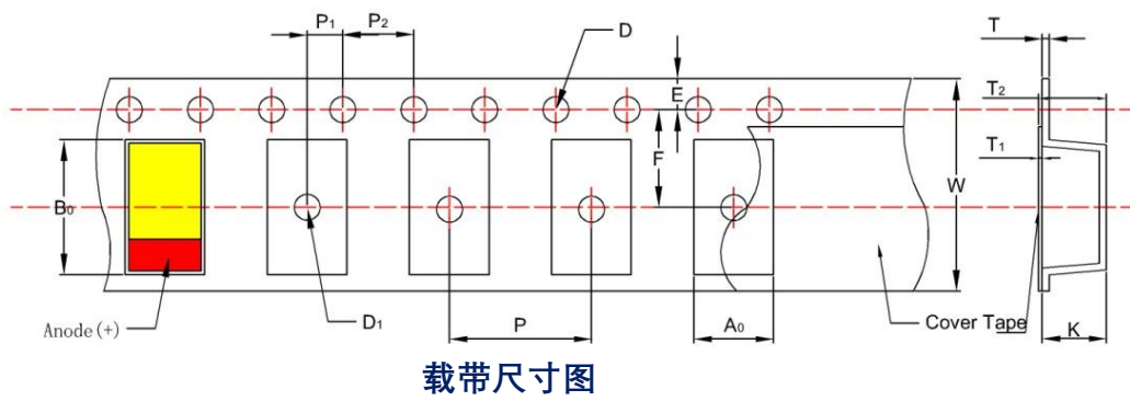
载带尺寸
