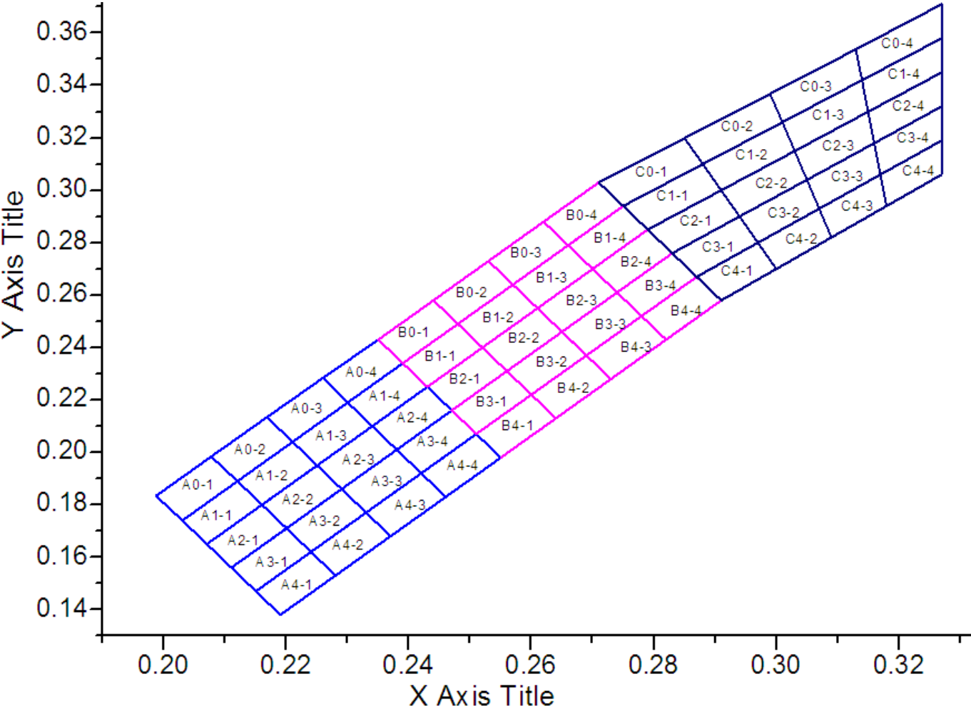
Chromaticity Diagram 1
