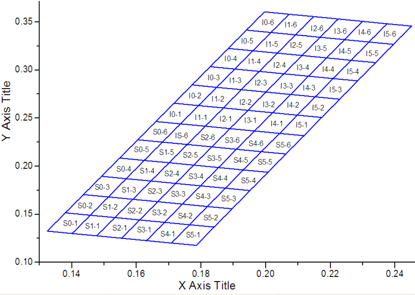
Chromaticity Diagram 2
