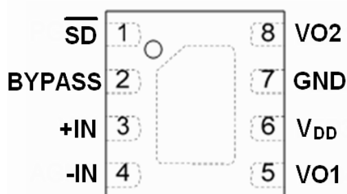
ft690V DFN3X3-8L (Top View)
