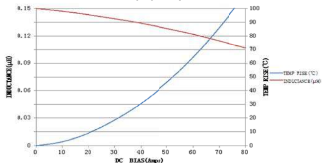
FXL1040-R15-M
