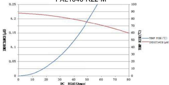
FXL1040-R22-M
