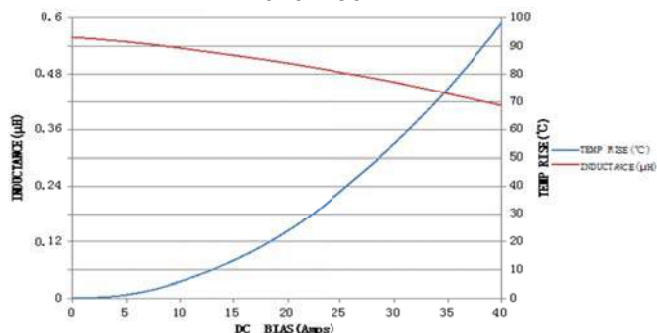
FXL1040-R56-M
