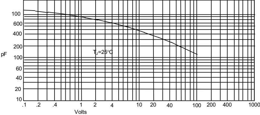
Figure 3 Junction Capacitance
